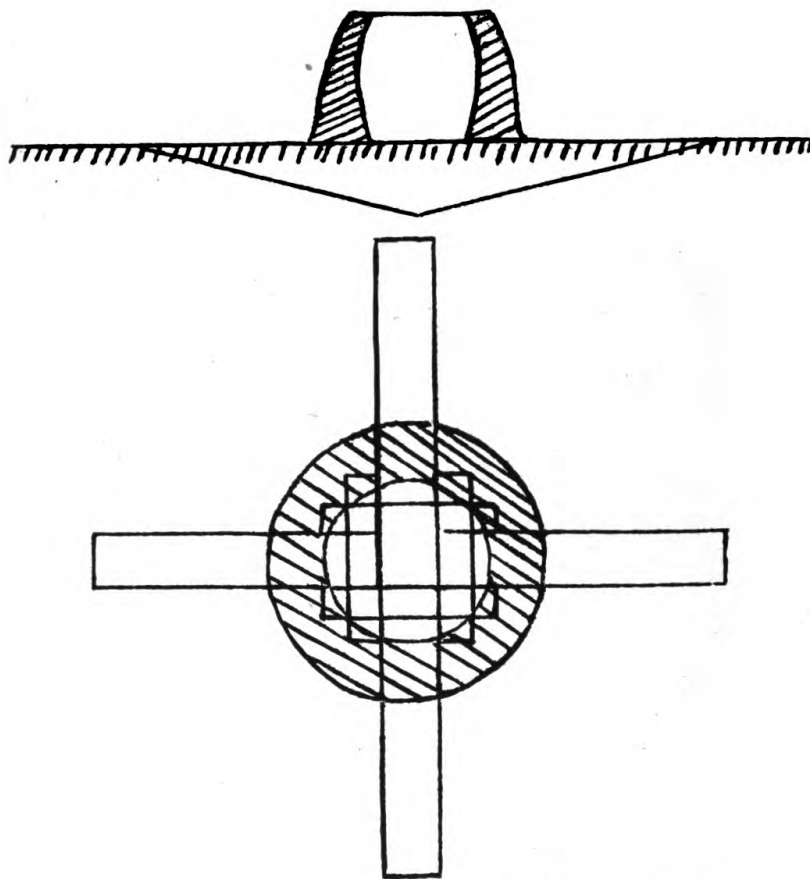
FIGURE 44.—Plan and cross section of company incinerator.
